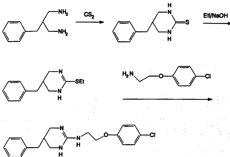
Scheme 19
